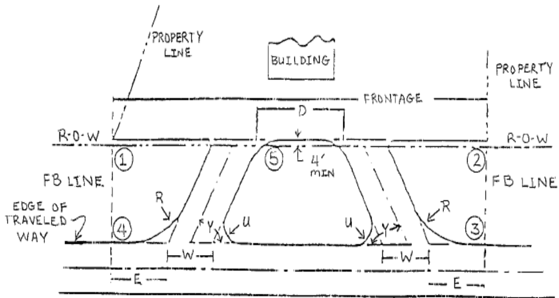
DOUBLE DRIVEWAY --- DIAGRAMMATIC FIGURE 2
