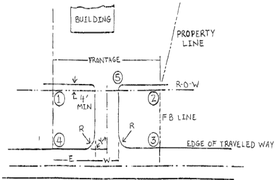
SINGLE DRIVEWAY --- DIAGRAMMATIC FOR ILLUSTRATING DEFINITIONS FIGURE 1
