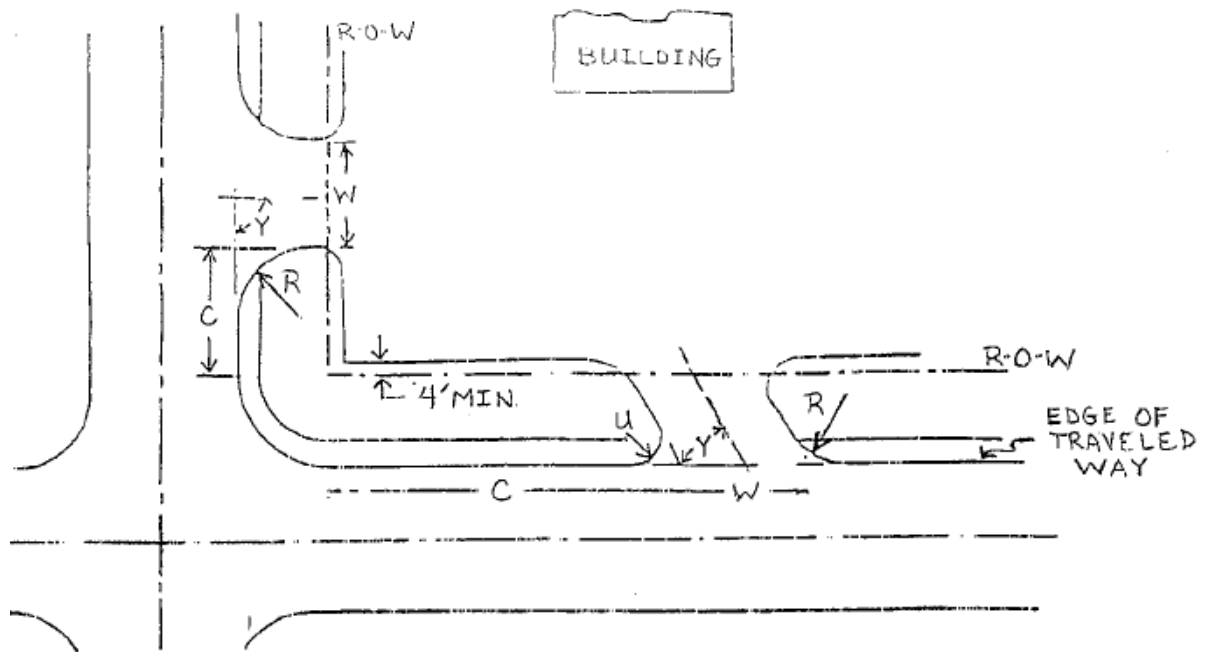
DRIVEWAYS FOR CORNER INSTALLATIONS DIAGRAMMATIC FIGURE 3
