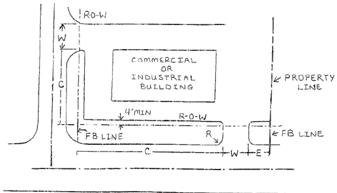
DRIVEWAYS TO A CORNER COMMERCIAL ESTABLISHMENT FIGURE 4
